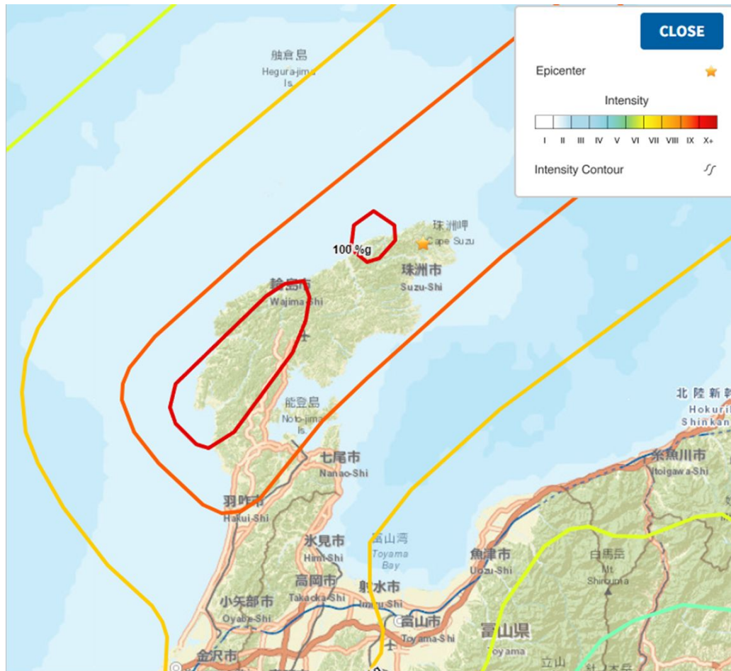
ShakeMap of the Noto Peninsula Earthquake with Peak Ground Acceleration (PGA) Source: United States Geological Survey (USGS)
